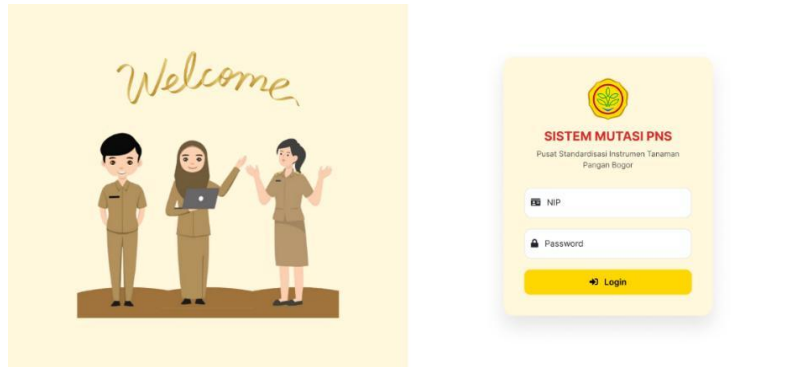
Figure 4. Login Page
